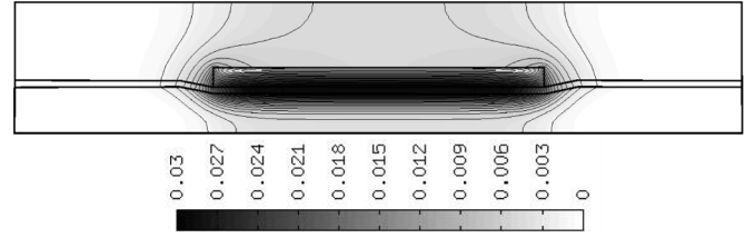
Fig. 3. Distribution of the module of magnetic flux density |\mathbf{B}| (T) in the system (practically independent of time t ).
