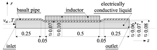
Fig. 1. Investigated arrangement (all dimensions are in m).
